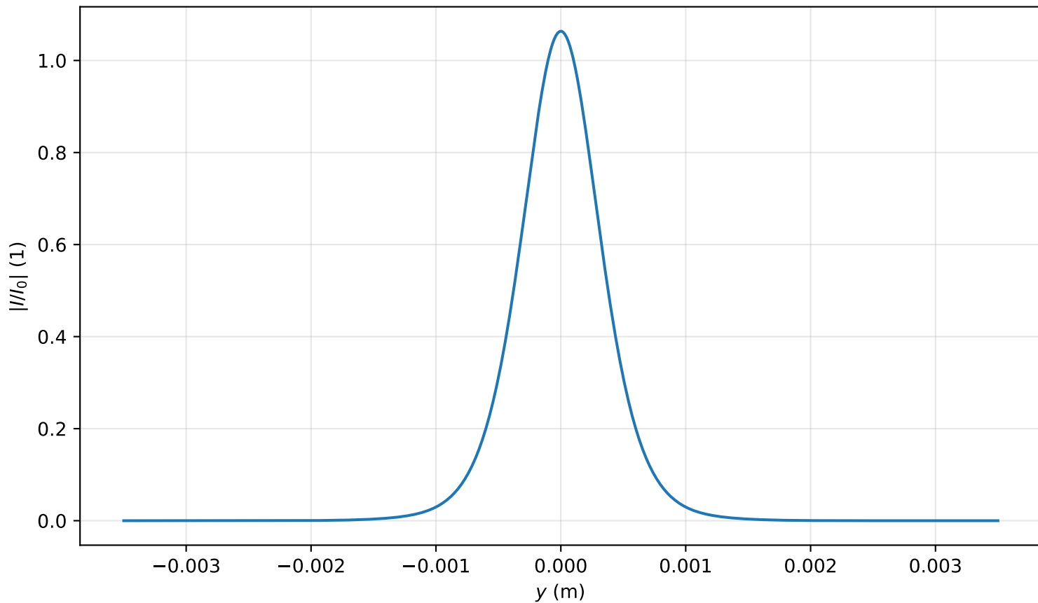
Intensity profile I(x=0, y, z=2.149)/I_0 , \text{Pin}=0.7\text{Pcr} , artificial time
